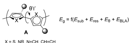
Figure 1. Structural factors determining the band gap of \pi -conjugated systems.
